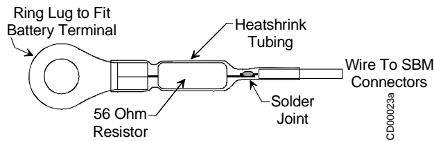
Fig. 1 Lead termination at battery cell.
