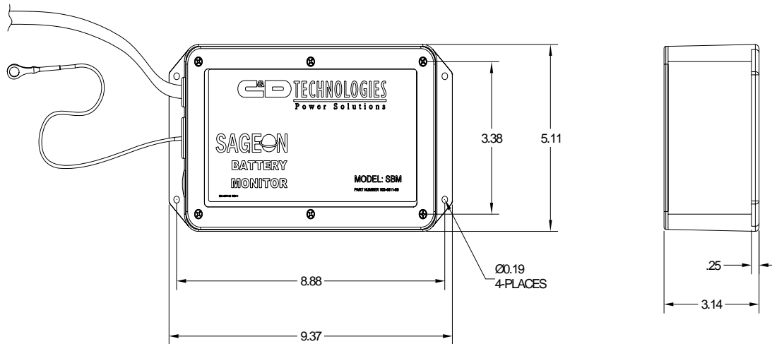
Fig. 3 SBM mounting hole locations.
