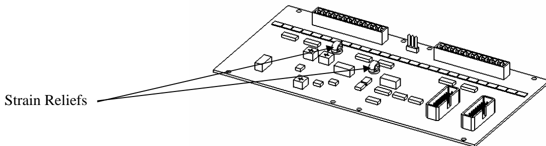
Fig. 2 Strain Relief locations.
